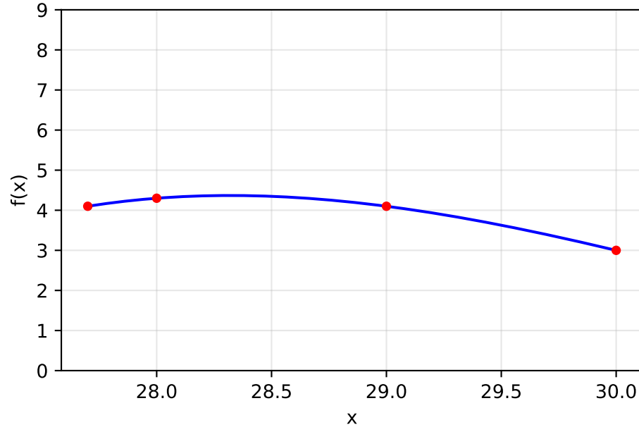
Curva 3: Vandermonde
